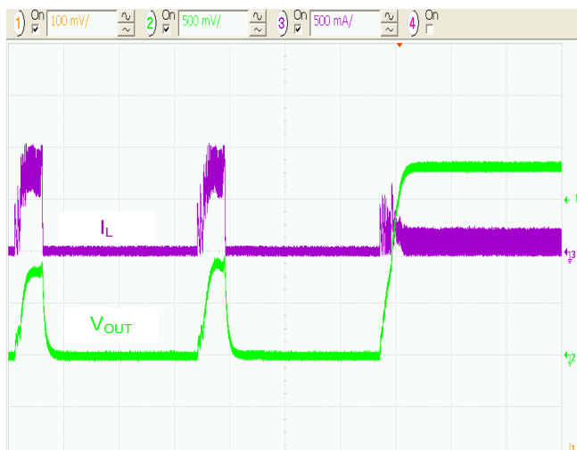
Figure 17. Overload Recovery to Light Load, 100μs/div.
