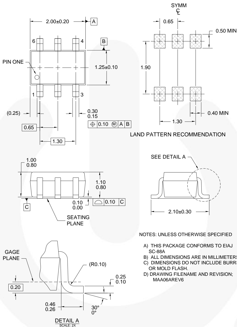
Figure 22. 6-Lead SC70
