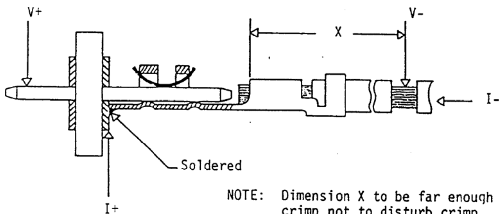
FIGURE 3 CONTACT RESISTANCE
