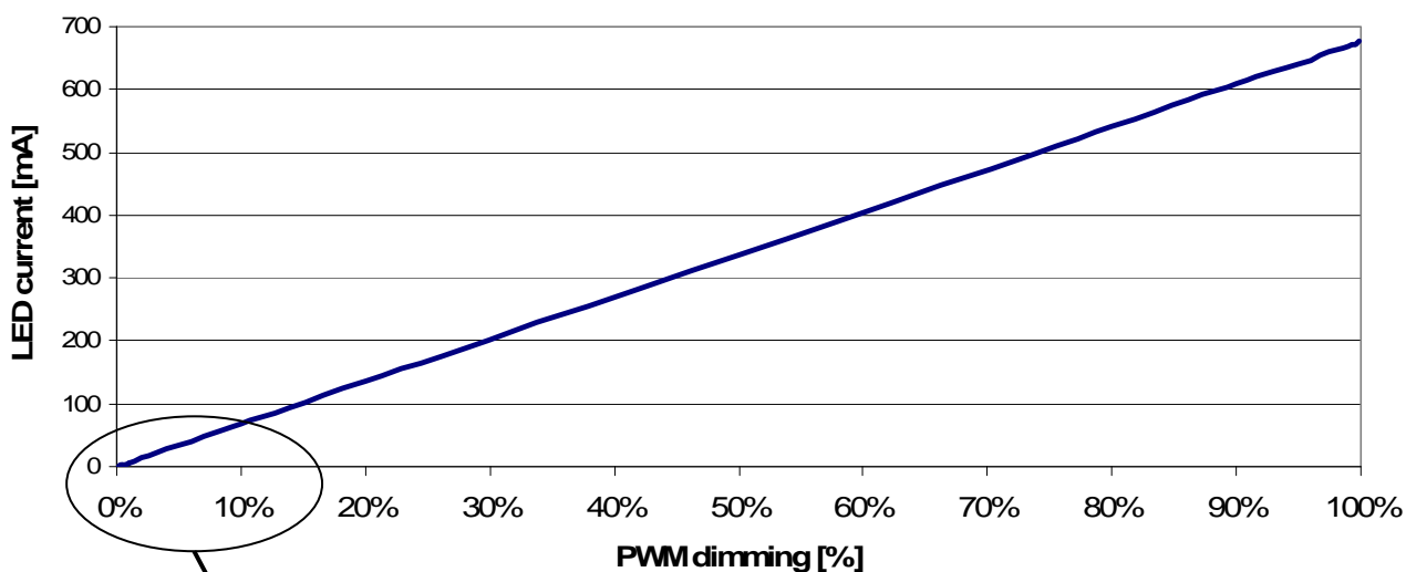
Figure 2 PWM Dimming at 500Hz
