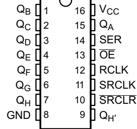
SN74LV595A ...D, DB, NS, OR PW PACKAGE (TOP VIEW)
