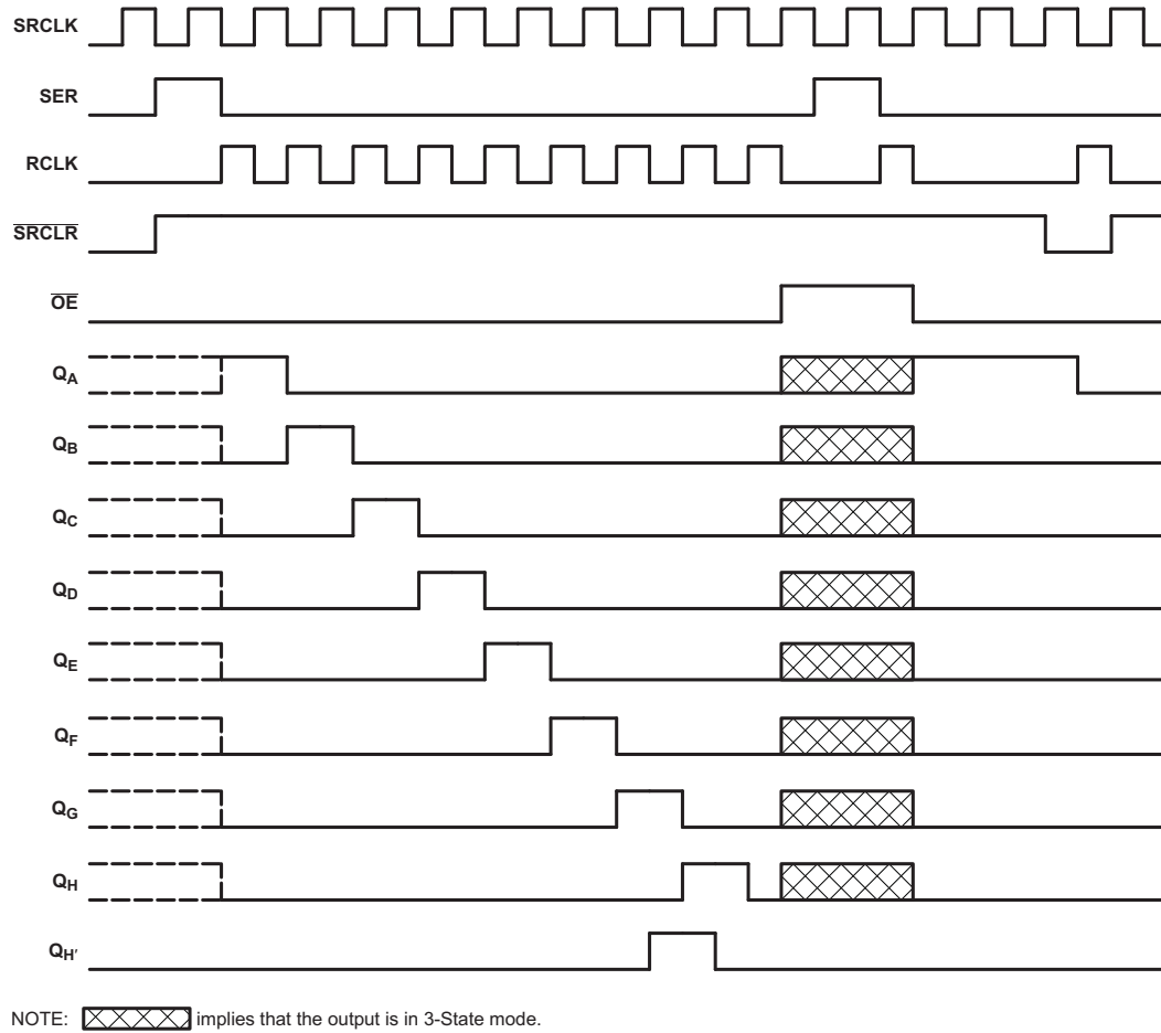
Figure 1. Timing Diagram
