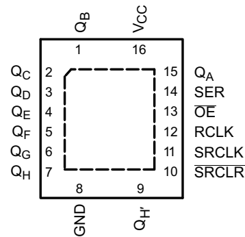
SN74LV595A ... RGY PACKAGE (TOP VIEW)
