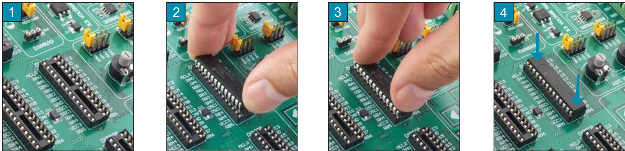
Figure 2-2: Plugging the microcontroller into appropriate socket
