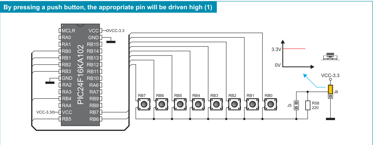
Figure 18-2: Microcontroller's PORTB and push buttons connection schematic
