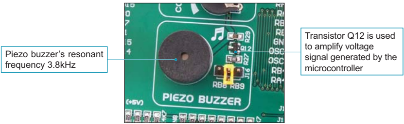
Figure 15-1: Piezo buzzer
