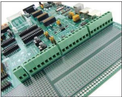
Figure 21-2: Screw connectors are connected to I/O pins
