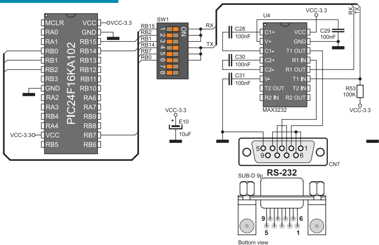
Figure 11-2: RS-232 module and microcontroller connection schematic
