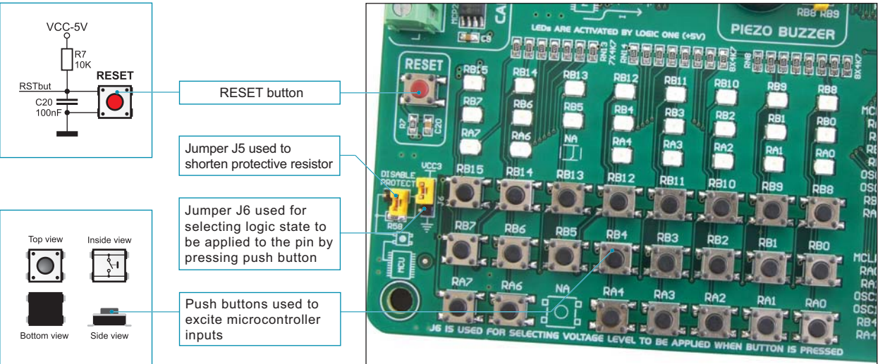
Figure 18-1: Push buttons
