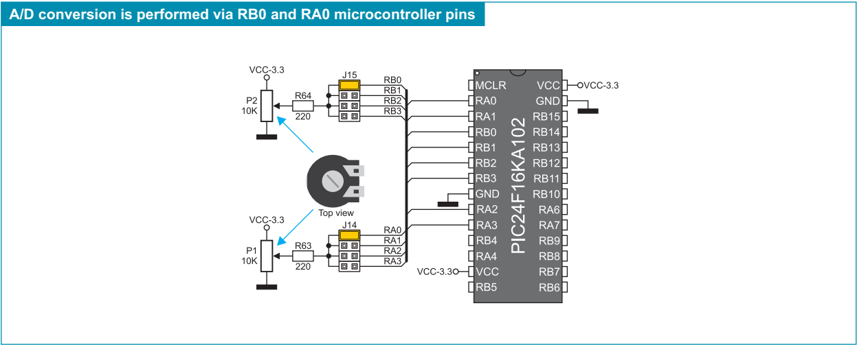
Figure 7-3: A/D converter test inputs and microcontroller connection schematic
