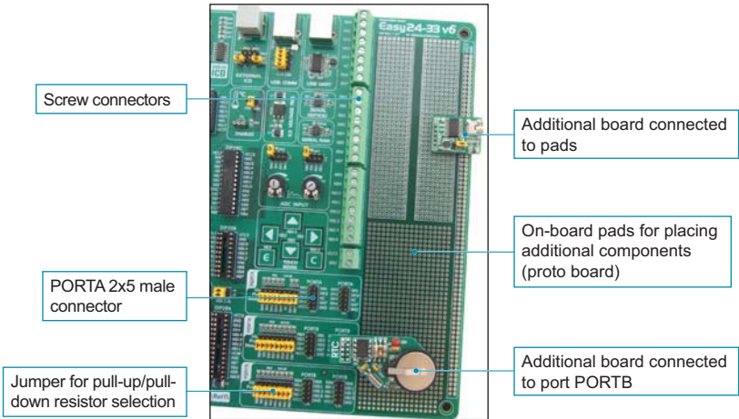
Figure 21-1: I/O ports
