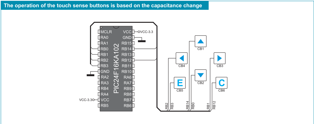
Figure 19-2: Touch sense keypad and microcontroller connection schematic
