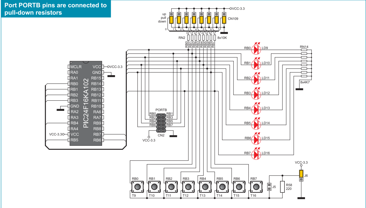
Figure 21-3: Port PORTB connection schematic
