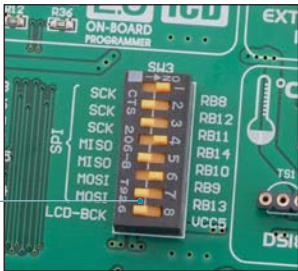
Figure 13-2: DIP switch SW3
