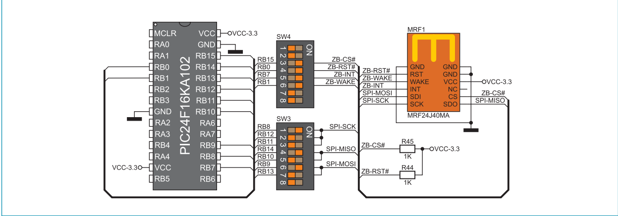
Figure 13-3: ZigBee module and microcontroller connection schematic
