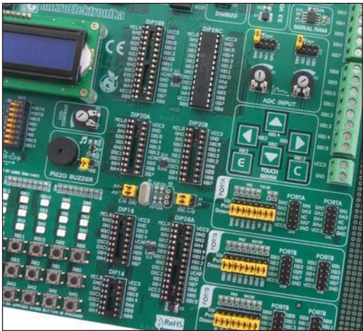
Figure 2-1: Microcontroller sockets
