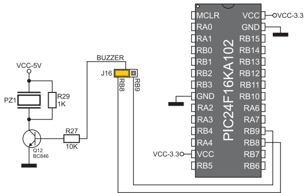
Figure 15-2: Piezo buzzer and microcontroller connection schematic
