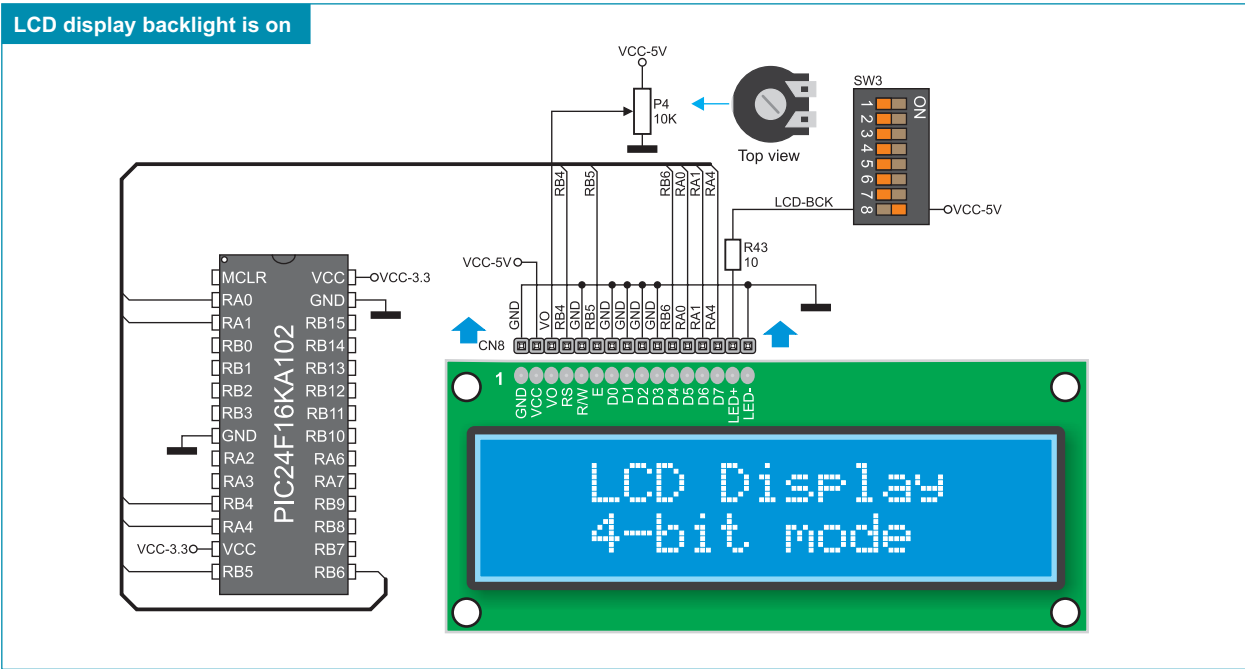
Figure 20-3. Alphanumeric 2x16 LCD and microcontroller connection schematic
