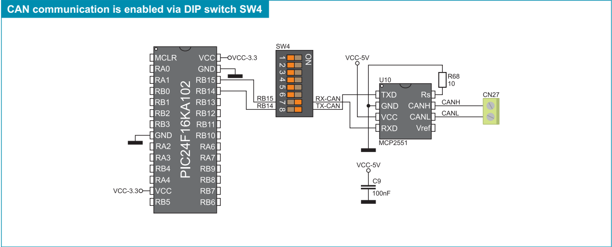
Figure 12-3: Microcontroller and CAN module connection schematic
