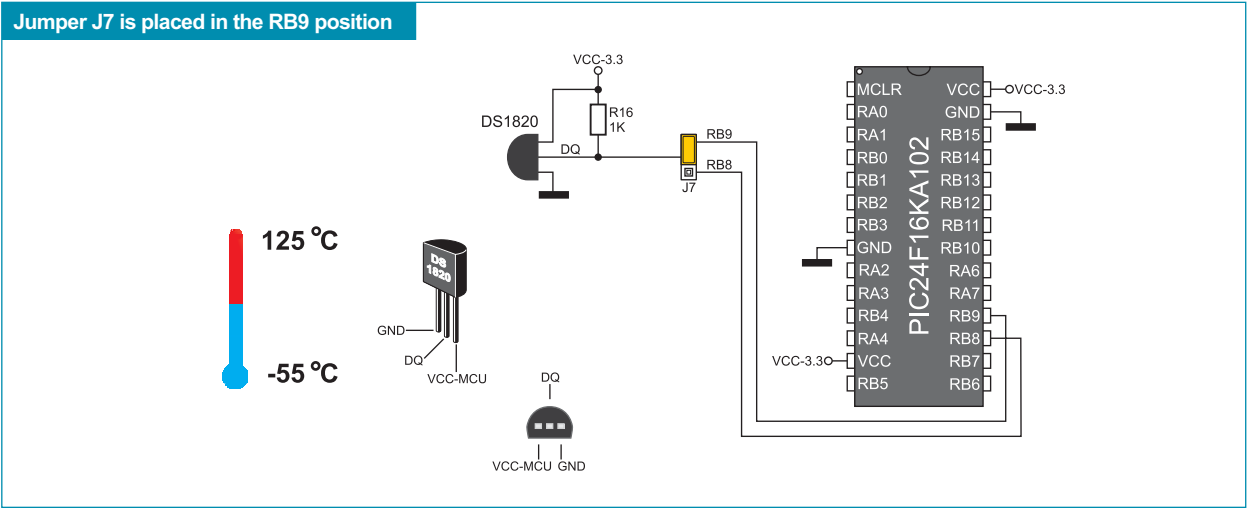
Figure 16-4: DS1820 temperature sensor and microcontroller connection schematic
