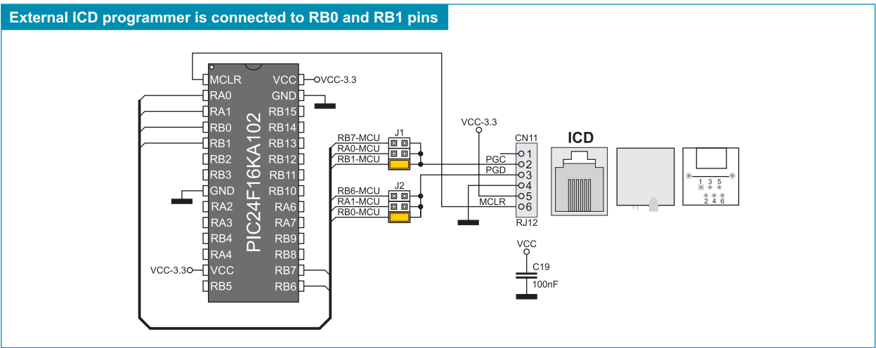
Figure 5-5: ICD connector and microcontroller connection schematic
