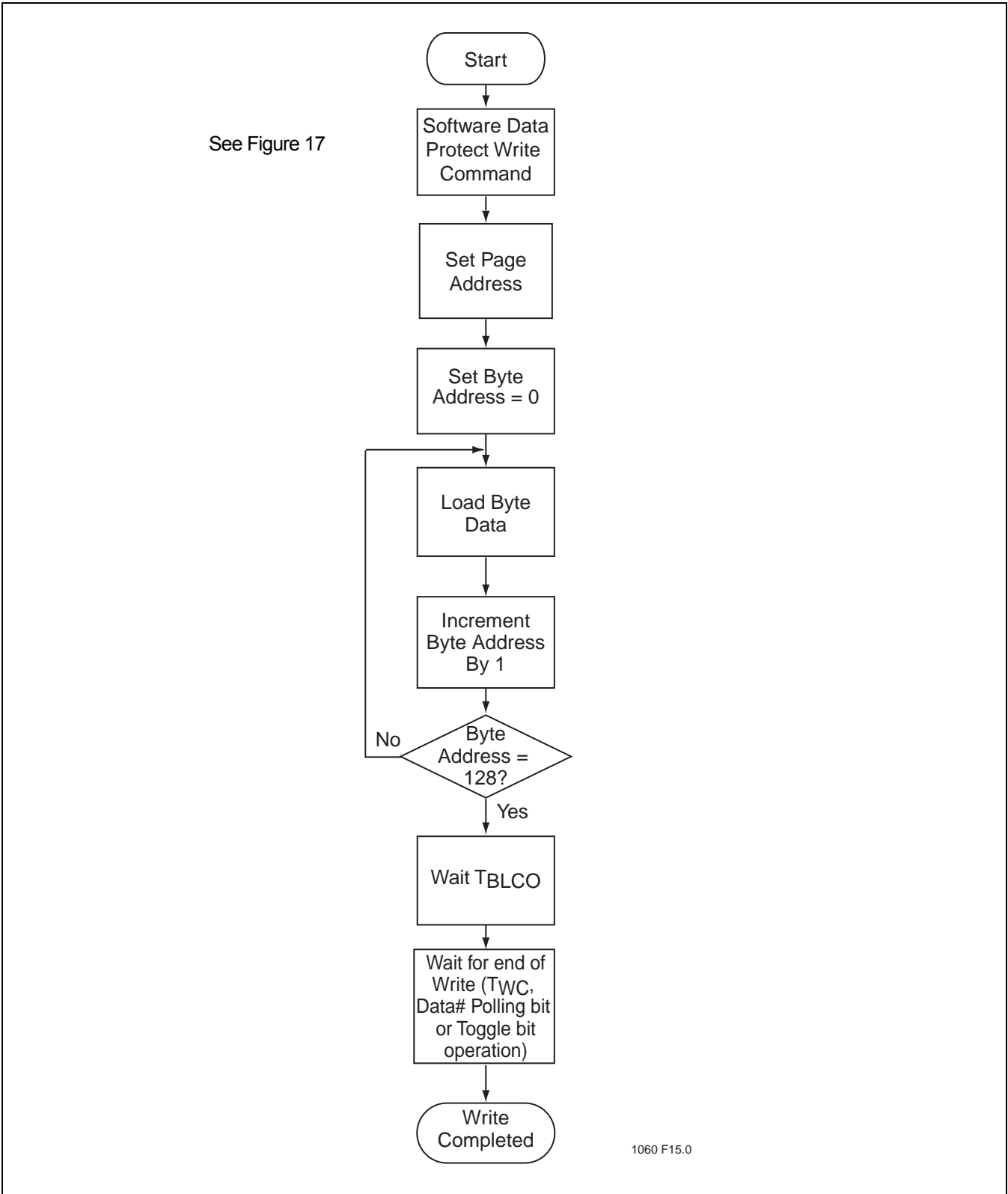
FIGURE 15: WRITE ALGORITHM
