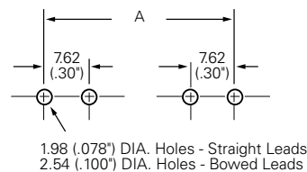
Recommended Mounting Dimensions
