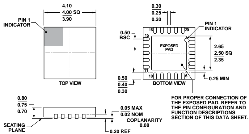
COMPLIANT TO JEDEC STANDARDS MO-220-WGGD. Figure 42. 20 Lead Lead Frame Chip Scale Package [LFCSP_WQ] 4 mm × 4 mm Body, Very Very Thin Quad (CP-20-10) Dimensions shown in millimeters
