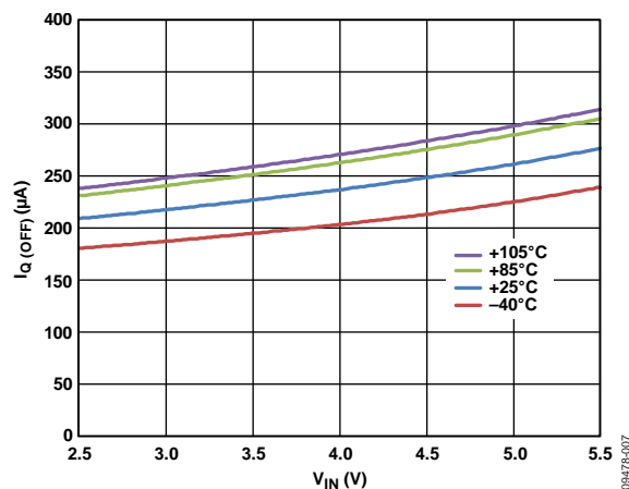
Figure 7. Typical Off Time Current ( I_{Q(\text{OFF})} )
