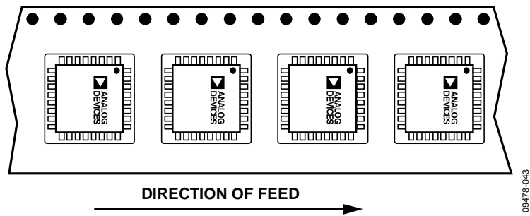
Figure 43. Tape and Reel Orientation for LFCSP Units
