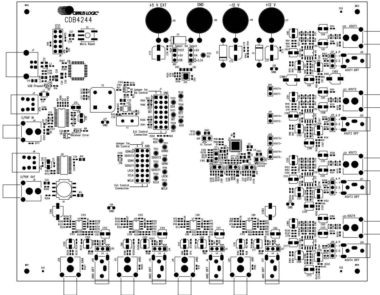
Figure 18. Silk Screen
