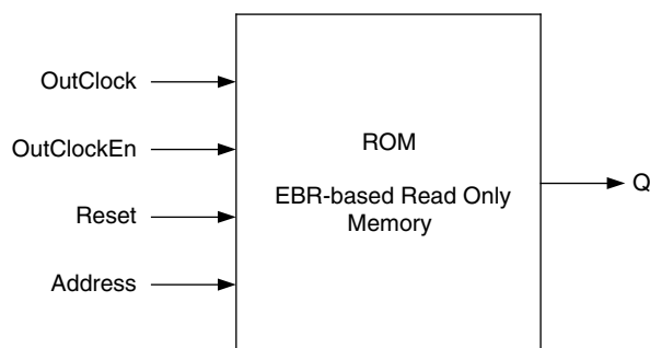
Figure 9-25. ROM – Read Only Memory Module Generated by IPexpress
