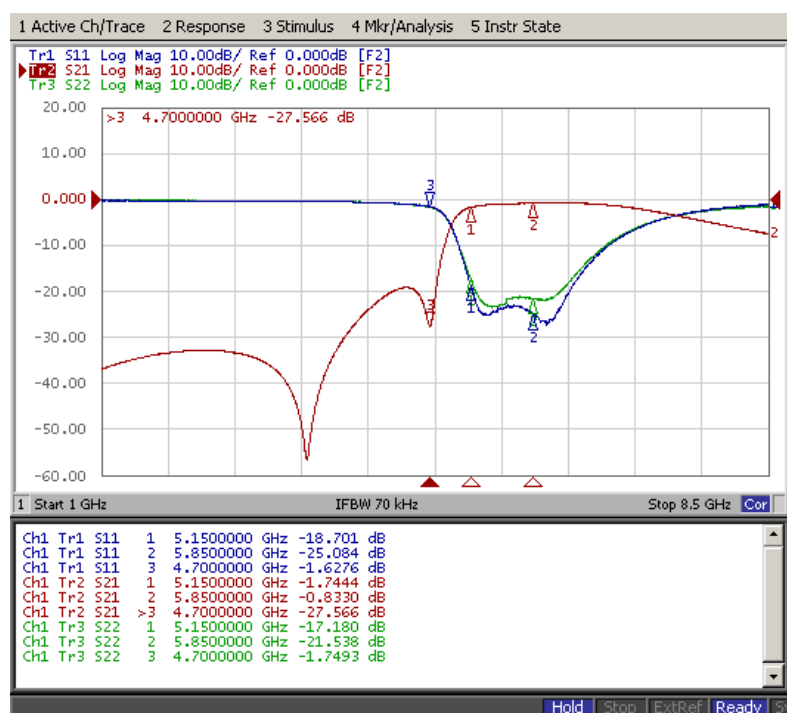
Fig. 3 Frequency Characteristics
