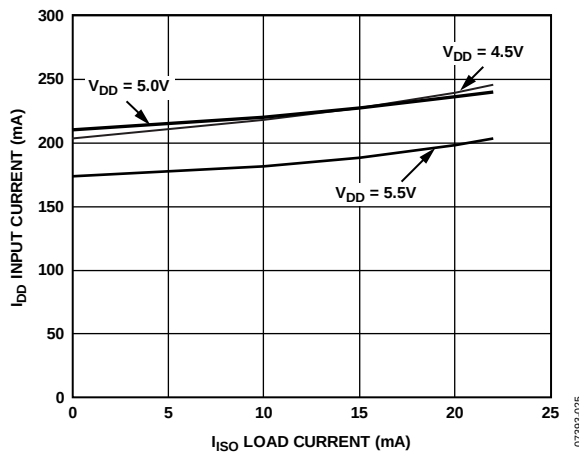
Figure 5. Typical I_{OD} Supply Current vs. I_{ISO} External Load
