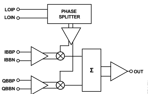
Figure 24. Block Diagram
