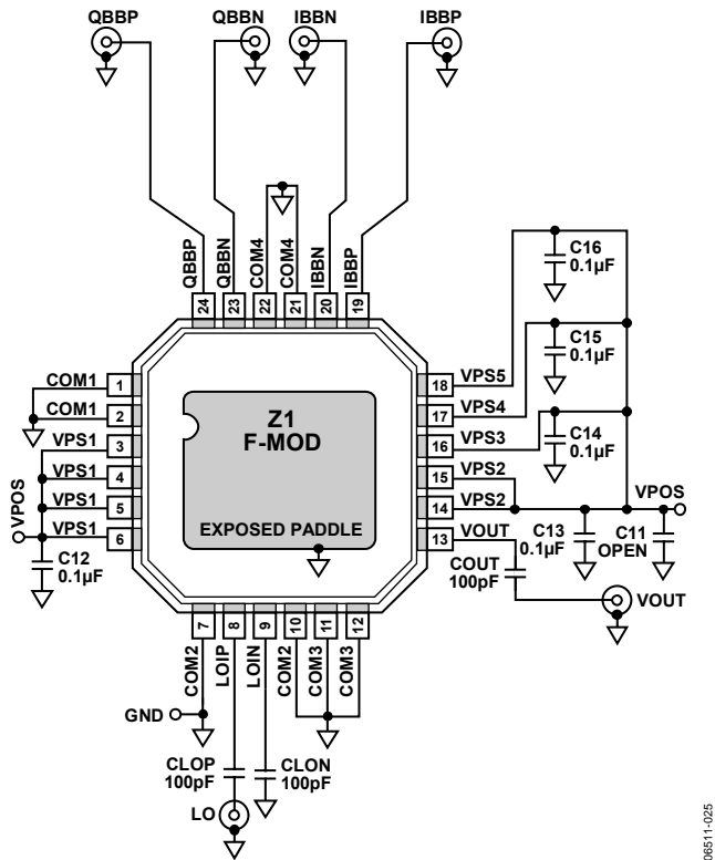
Figure 25. Basic Connections for the ADL5372
