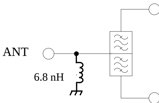
Fig. 2. Matching Circuit
