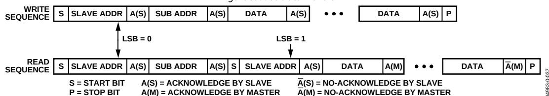
Figure 40. Read and Write Sequence
