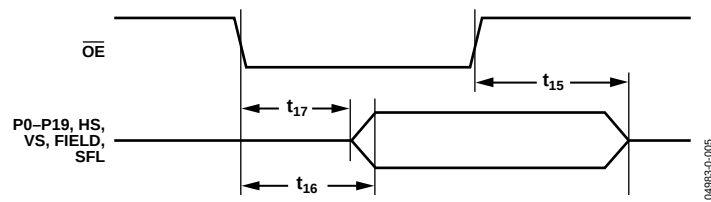
Figure 4. \overline{OE} Timing
