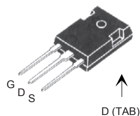
TO-247 (IXFH)
