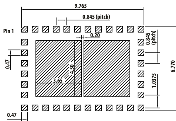
Stencil Opening
