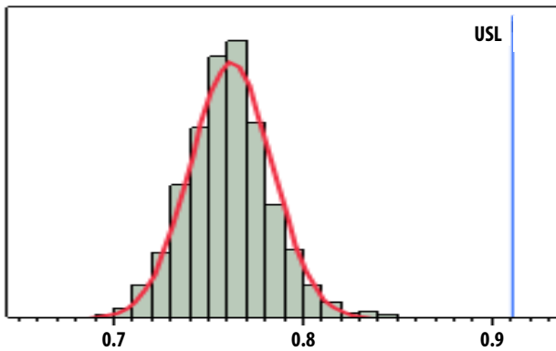
Figure 3. NF, nominal = 0.76 dB, USL = 0.91 dB
