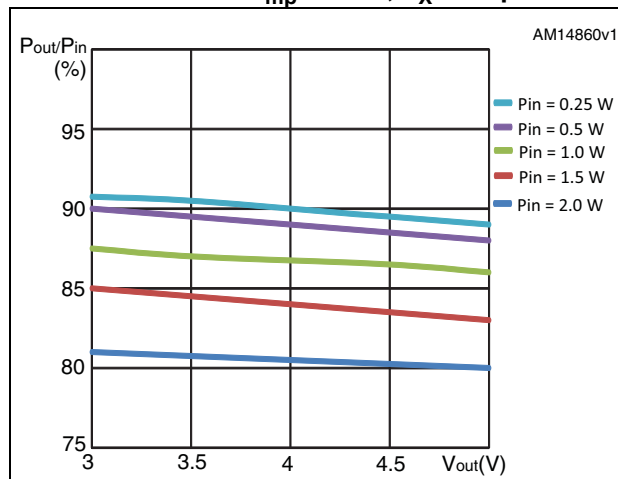
Figure 6. Efficiency vs output voltage 4 PV cells - V_{mp} = 2\text{ V} , L_X = 33\text{ }\mu\text{H}
