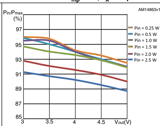
Figure 7. MPPT efficiency vs output voltage 4 PV cells - V_{mp} = 2\text{ V} , L_X = 33\text{ }\mu\text{H}
