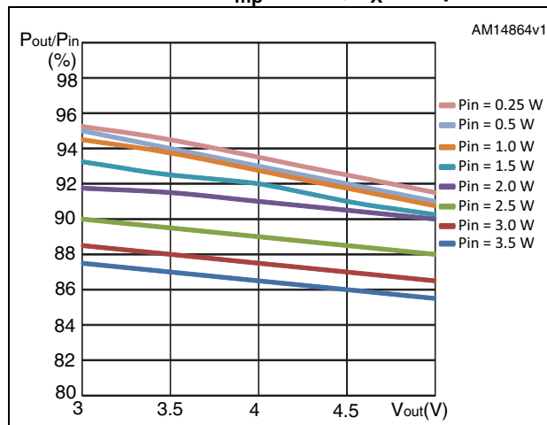
Figure 8. Efficiency vs output voltage 5 PV cells - V_{mp} = 2.5\text{ V} , L_X = 33\text{ }\mu\text{H}
