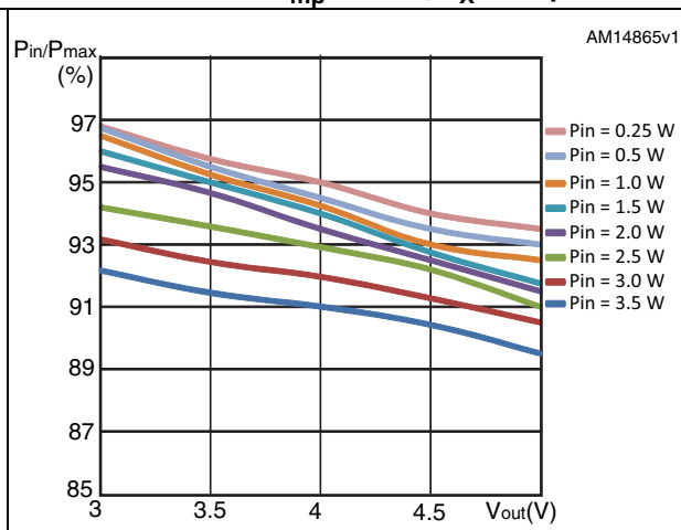
Figure 9. MPPT efficiency vs output voltage 5 PV cells - V_{mp} = 2.5\text{ V} , L_X = 33\text{ }\mu\text{H}
