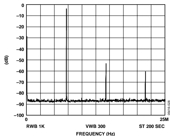
Figure 28. f_{MCLK} = 50 MHz, f_{OUT} = 7.143 MHz = f_{MCLK}/7 , Frequency Word = 249249
