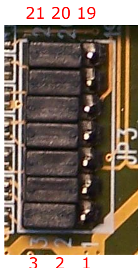
Figure 3 Setting termination and biasing resistors
