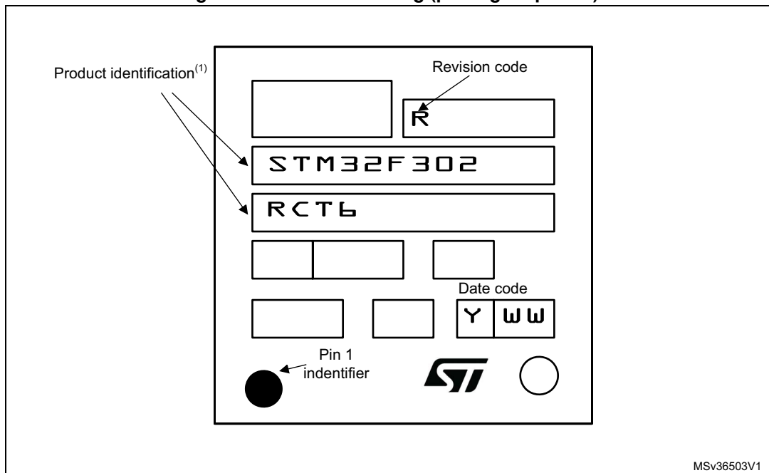
Figure 43. LQFP64 marking (package top view)
