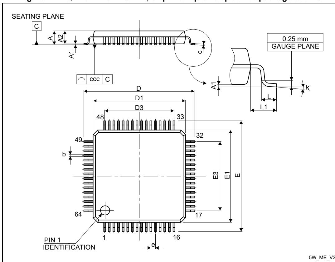
Figure 41. LQFP64 – 10 x 10 mm, 64 pin low-profile quad flat package outline
