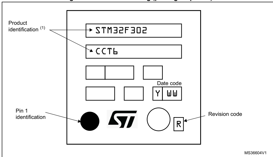
Figure 46. LQFP48 marking (package top view)
