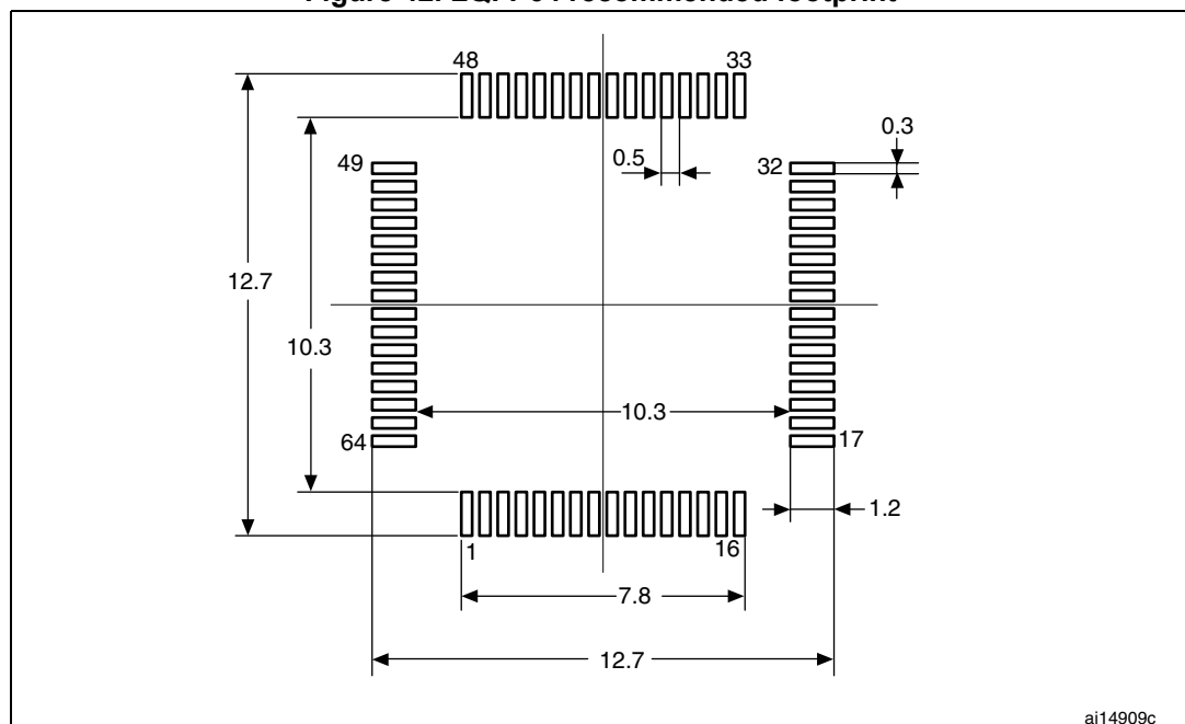
Figure 42. LQFP64 recommended footprint
