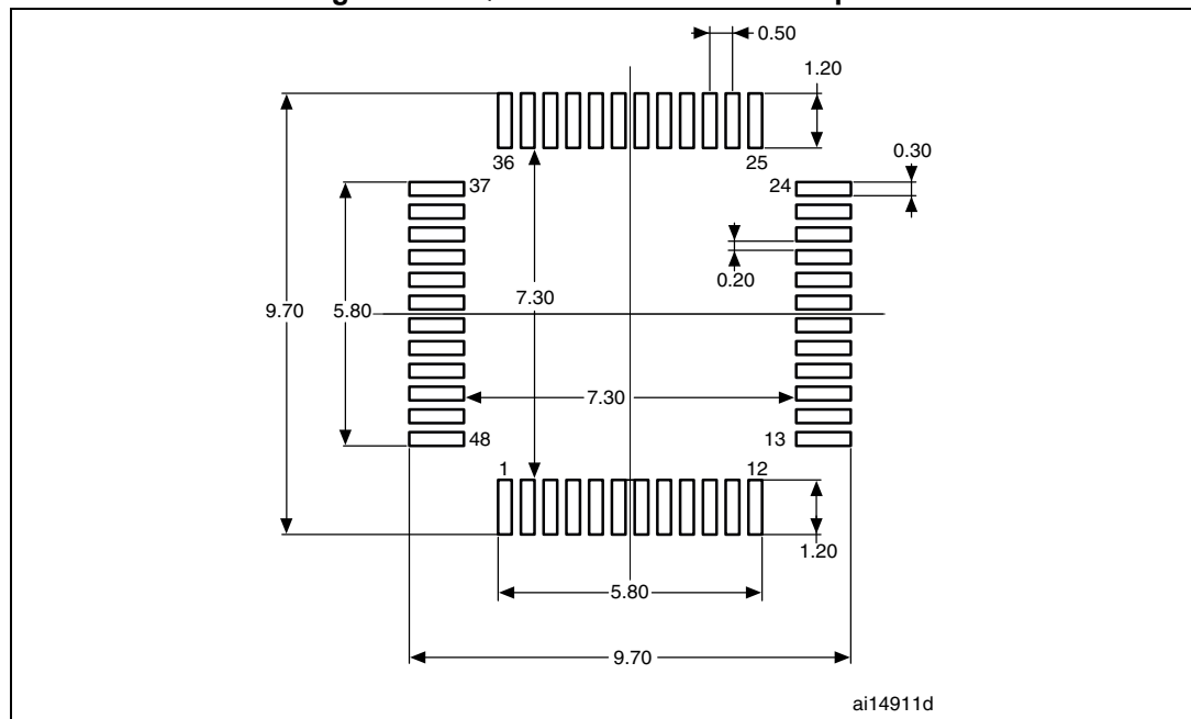
Figure 45. LQFP48 recommended footprint
