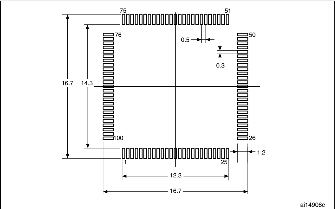
Figure 39. LQFP100 recommended footprint
