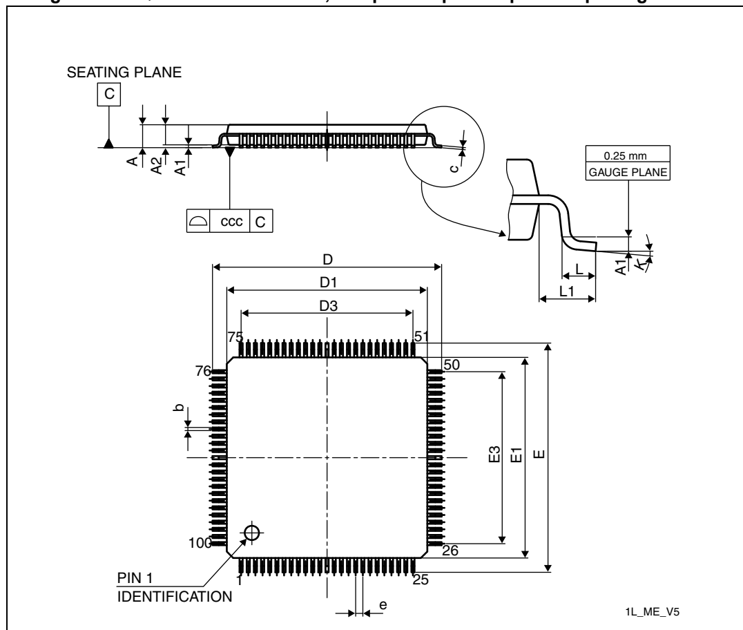
Figure 38. LQFP100 – 14 x 14 mm, 100-pin low-profile quad flat package outline
