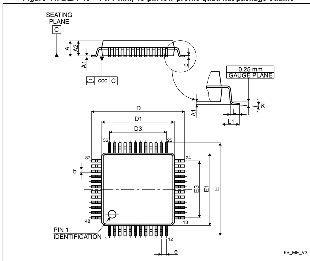
Figure 44. LQFP48 – 7 x 7 mm, 48-pin low-profile quad flat package outline
