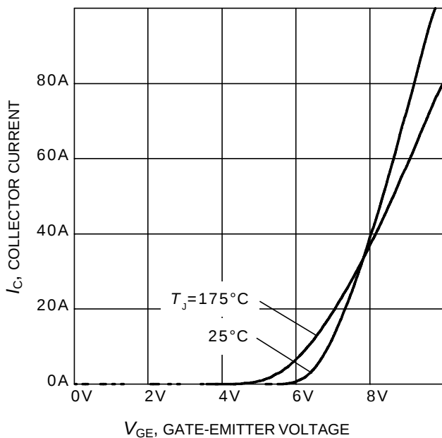
Figure 7. Typical transfer characteristic ( V_{CE}=10V )
