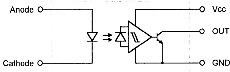
Figure 1. INTERNAL CONNECTIONS
