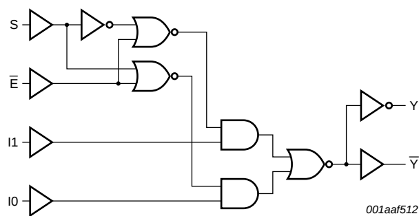
Fig 4. Functional diagram
