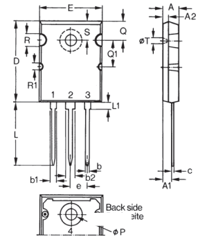
TO-264 (IXTK) Outline
