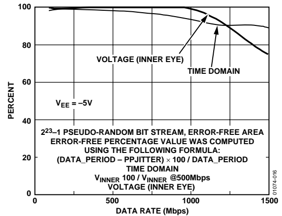
Figure 16. AC Performance
