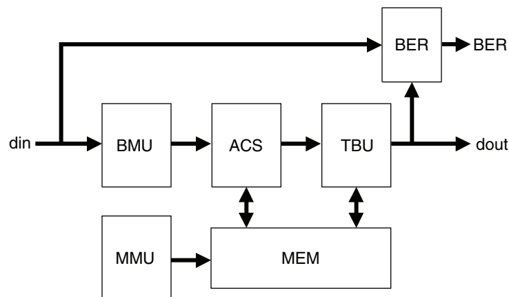
Figure 2-6. Internal Architecture of the Viterbi Decoder
