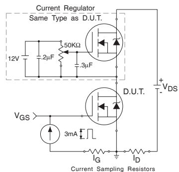
Fig 13b. Gate Charge Test Circuit www.irf.com
