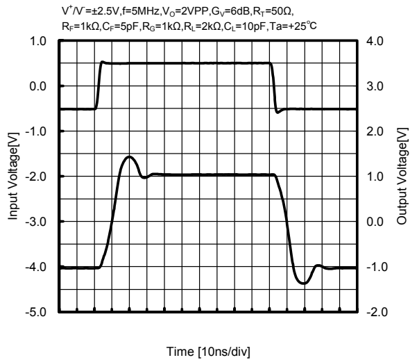
Pulse Response
