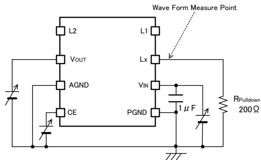
< Circuit No.⑤ >
