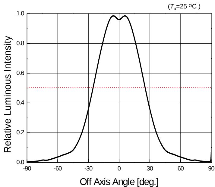
Radiation Diagram
