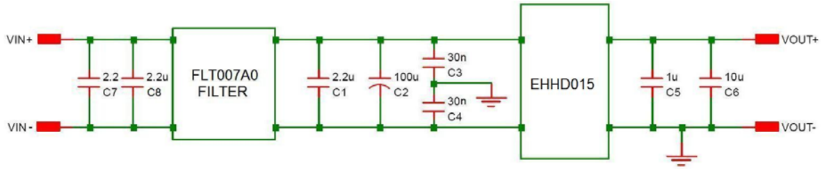
Figure 29. EMC Considerations
