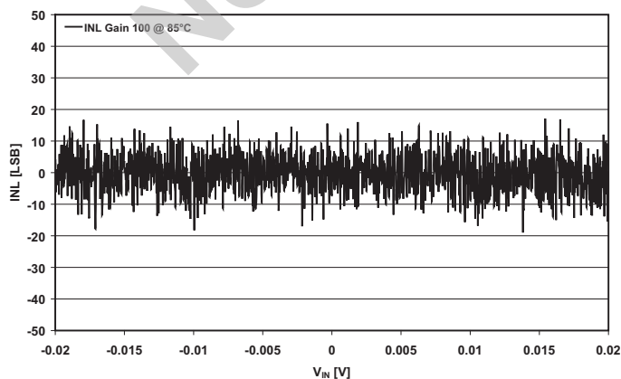
Figure 39. INL 85°C
