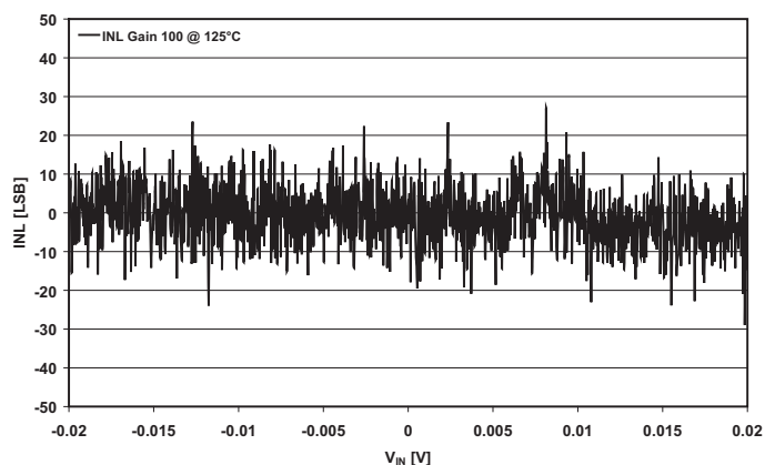
Figure 40. INL 125°C
