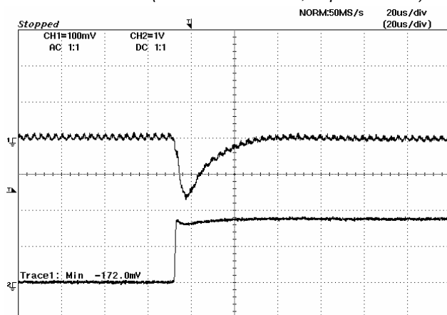
Figure 24: Typical transient response to step load change at 2.5A/μS from 50% to 100% of I_o , max at 3.3Vin, 2.5Vout (Cout = 1uF ceramic, 10μF tantalum)
