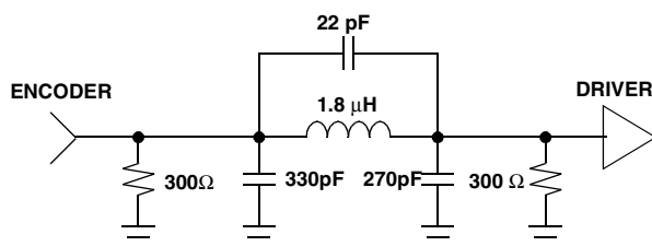
Figure 3. 300 Ω Filters
