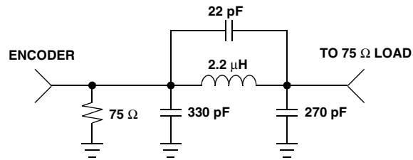
Figure 4. 75 Ω Filters
