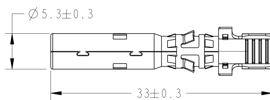
SOCKET (FEMALE)
