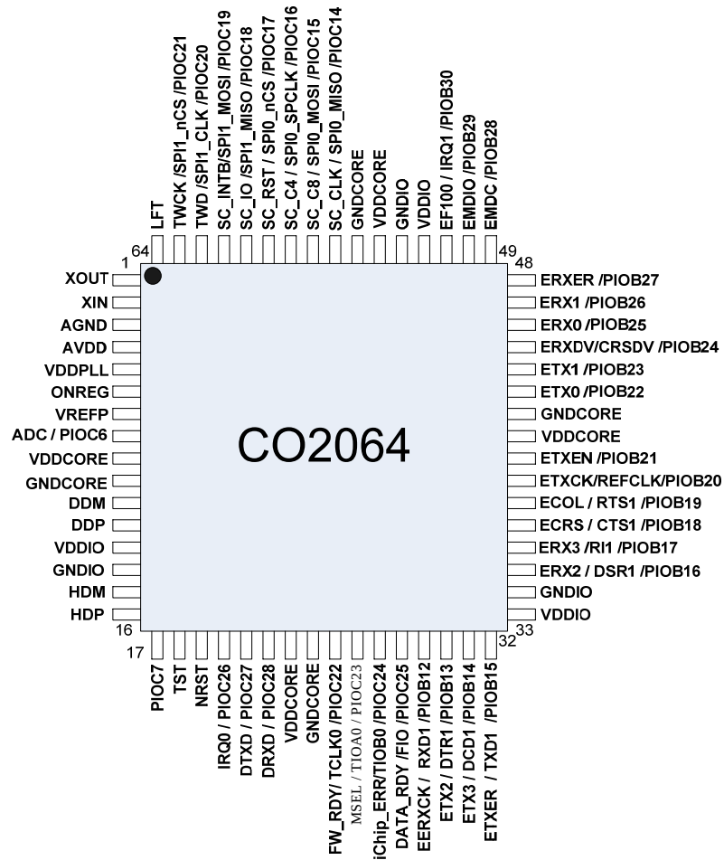
Figure 3-6: Pin-out for the 64-pin Package
