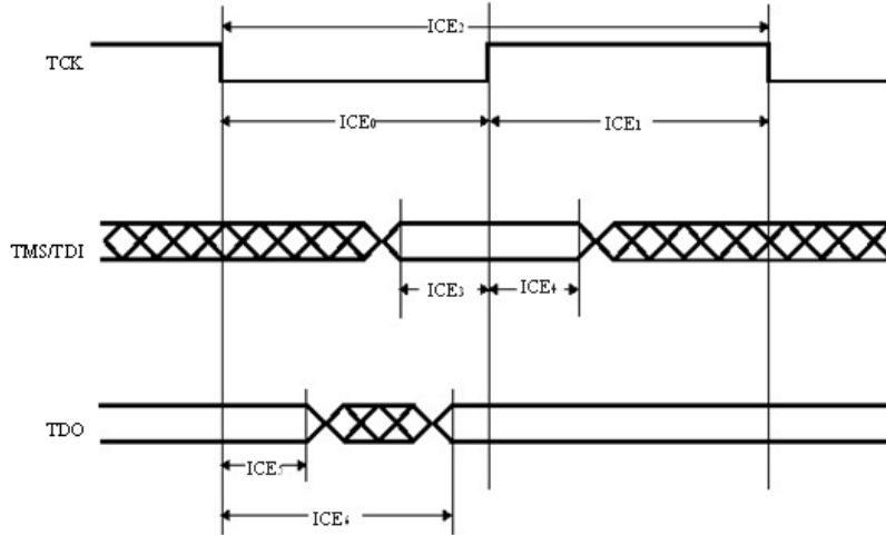
Figure 8-4: ICE Timings
