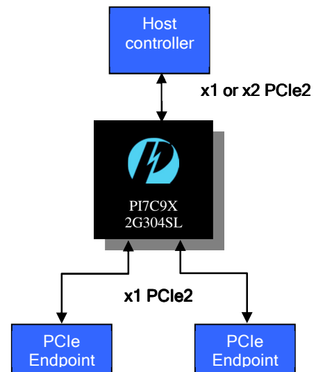
PI7C9X2G304SL – Application Example
