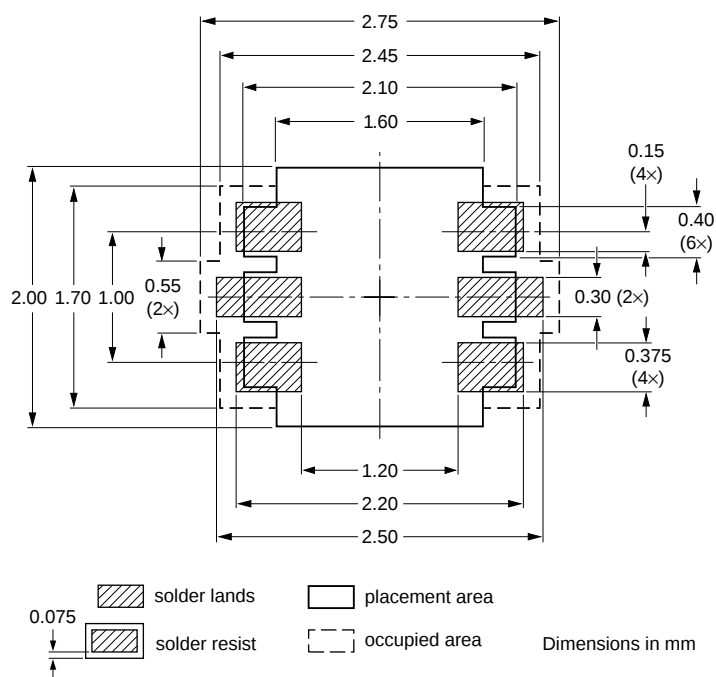
Fig 7. Reflow soldering footprint SOT666
