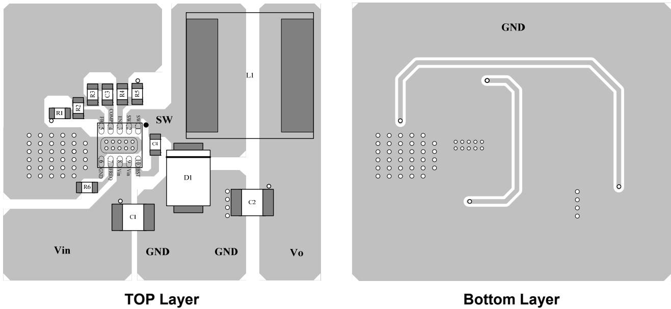
Figure 6—MP2562 Typical Application Circuit and PCB Layout Guide
