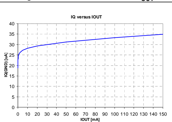
Figure 11. Quiescent current vs. I_{OUT}
