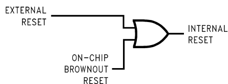
Figure 8. Reset Logic
