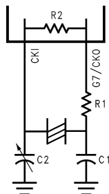
Figure 12. High-Speed Crystal Oscillator
