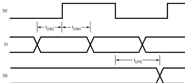
Figure 2. MICROWIRE/PLUS Timing
