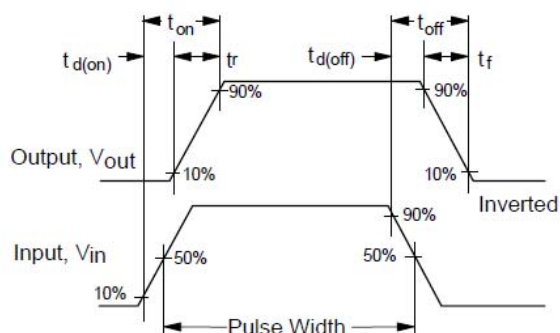
Figure 12. Switching Waveforms.
