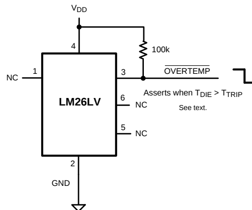
Figure 24. Temperature Switch Using Open-Drain Output
