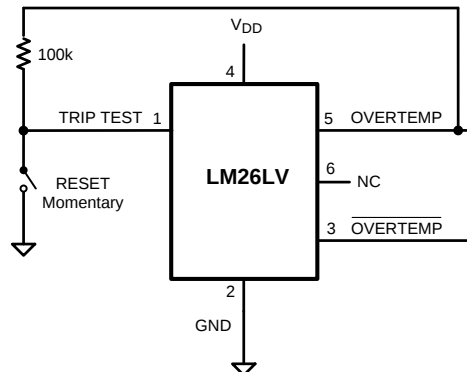
Figure 28. Latch Circuit using OVERTEMP Output
