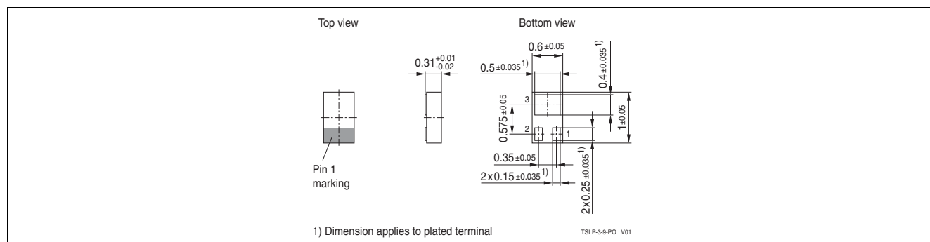
Figure 7-1 Package Outline
