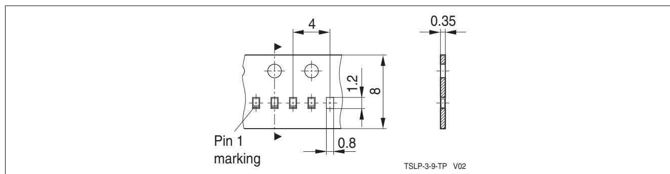
Figure 7-4 Tape Dimensions
