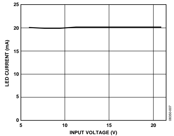
Figure 7. LED Current vs. Input Voltage ( I_{LED} = 20\text{mA} )
