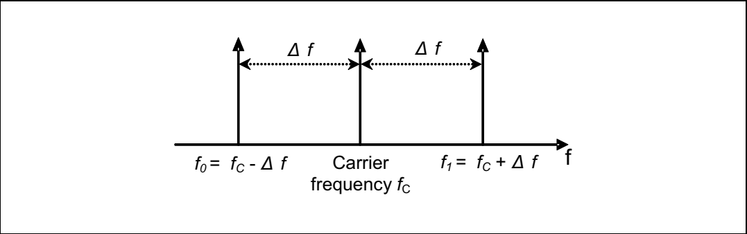
Figure 13. Frequency deviation
