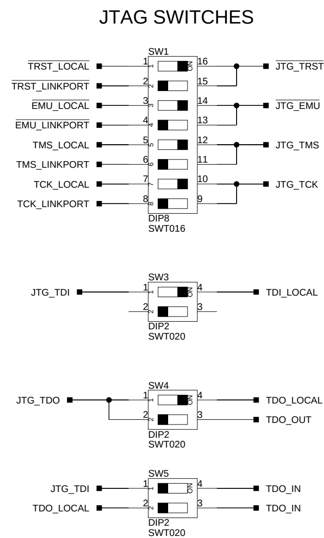
MULTI PROCESSOR JTAG SETTINGS VIA HP-USB EMUALTOR USING TWO OR MORE EZ-BOARDS (LINK PORT CABLES REQUIRED FOR MORE THAN TWO BOARDS)
