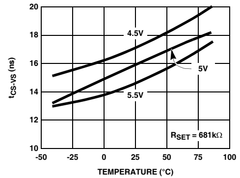
FIGURE 16. COMPOSITE SYNC TO VERTICAL SYNC DELAY TIME
