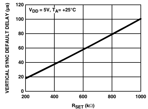
FIGURE 10. VERTICAL DEFAULT DELAY vs RSET
