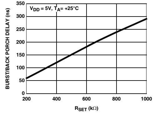
FIGURE 8. BURST/BACK PORCH DELAY vs RSET
