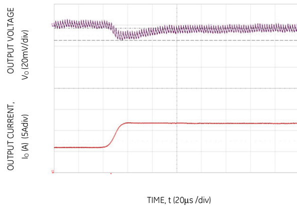
Figure 4. Transient Response to Dynamic Load Change from 50% to 100% on one output at 12Vin, C out =2×47μF+7×330μF, C Tune =12nF, R Tune =300Ω
