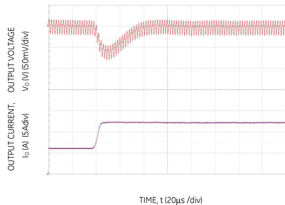
Figure 28. Transient Response to Dynamic Load Change on one output from 50% to 100% at 12V in , C_{out} = 3 \times 47\mu\text{F} + 1 \times 330\mu\text{F} , C_{Tune} = 1200\text{pF} & R_{Tune} = 300\Omega
