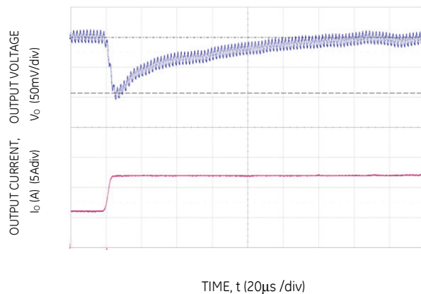
Figure 34. Transient Response to Dynamic Load Change on one output from 50% to 100% at 12Vin, C_{out} = 6 \times 47\mu\text{F} , C_{Tune} = 470\text{pF} & R_{Tune} = 300\Omega
