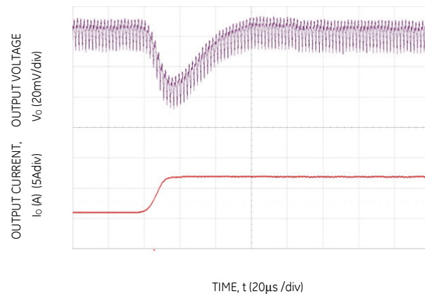
Figure 16. Transient Response to Dynamic Load Change on one output from 50% to 100% at 12Vin, C_{out} = 3 \times 47\mu F + 2 \times 330\mu F , C_{Tune} = 1800pF & R_{Tune} = 300\Omega
