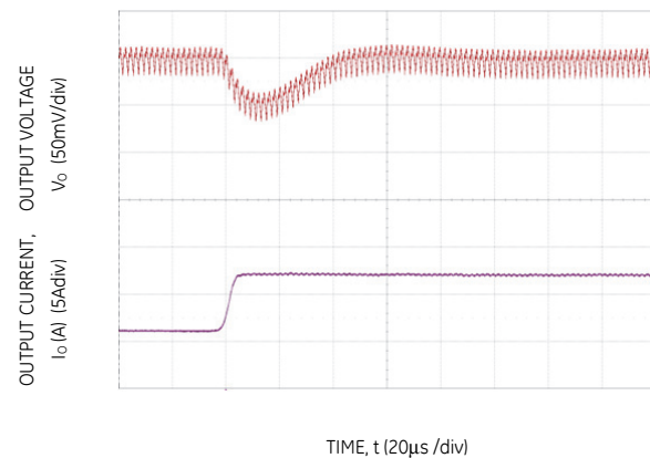
Figure 22. Transient Response to Dynamic Load Change on one output from 50% to 100% at 12V in , C_{out} = 3 \times 47\mu\text{F} + 2 \times 330\mu\text{F} , C_{Tune} = 1500\text{pF} & R_{Tune} = 300\Omega
