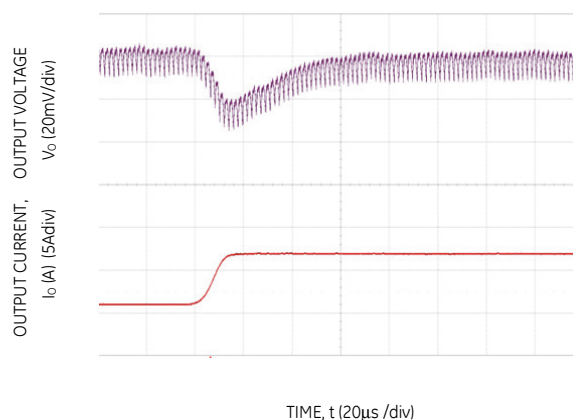
Figure 10. Transient Response to Dynamic Load Change on one output from 50% to 100% at 12V in , C_{out} = 3 \times 47\mu\text{F} + 3 \times 330\mu\text{F} , C_{Tune} = 2700\text{pF} & R_{Tune} = 300\Omega
