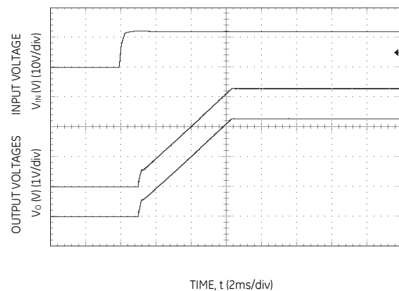
Figure 30. Typical Start-up Using Input Voltage ( V_{IN} = 12\text{V} , I_o = I_{o1,max}, I_{o2,max} ).
