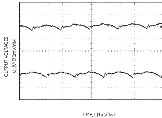
Figure 3. Typical output ripple and noise (C o = 2×0.1μF+2×47μF ceramic, V IN = 12V, I o = I o1,max , I o2,max ).
