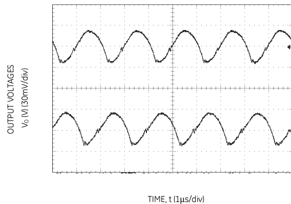
Figure 27. Typical output ripple and noise ( C_o = 2 \times 0.1\mu\text{F} + 2 \times 47\mu\text{F} ceramic, V_{IN} = 12\text{V} , I_o = I_{o1,max}, I_{o2,max} ).
